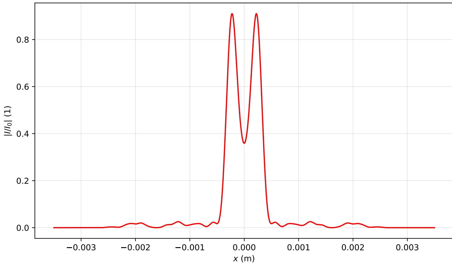
Intensity profile I(x, y = 0, z = 2.627)/I_0 , P_{in}=3.5P_{cr} , artificial time
